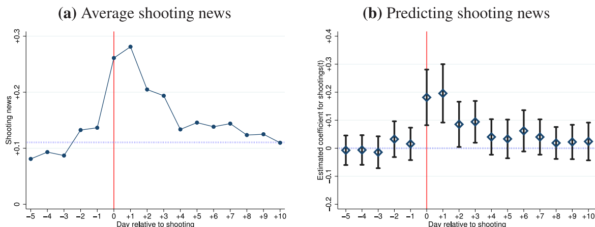
Fig. 1. Left : Shooting news around shooting days, where the dashed horizontal line indicates the sample average of 0.11. Right : Estimates from regressing shooting news on day t on 16 variables for the number of shootings on days t - 5 until t + 10 , while controlling for a linear and squared time trend, as well as fixed effects for each weekday, month, and year.
