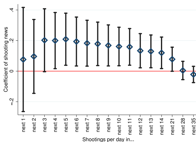
Fig. 4. Predicted additional shootings for various time frames of the dependent variable. Each point represents one IV regression outcome, and all regressions include the control variables presented in Eq. (1) and Table 4. Two-sided 95 percent confidence intervals are displayed.
