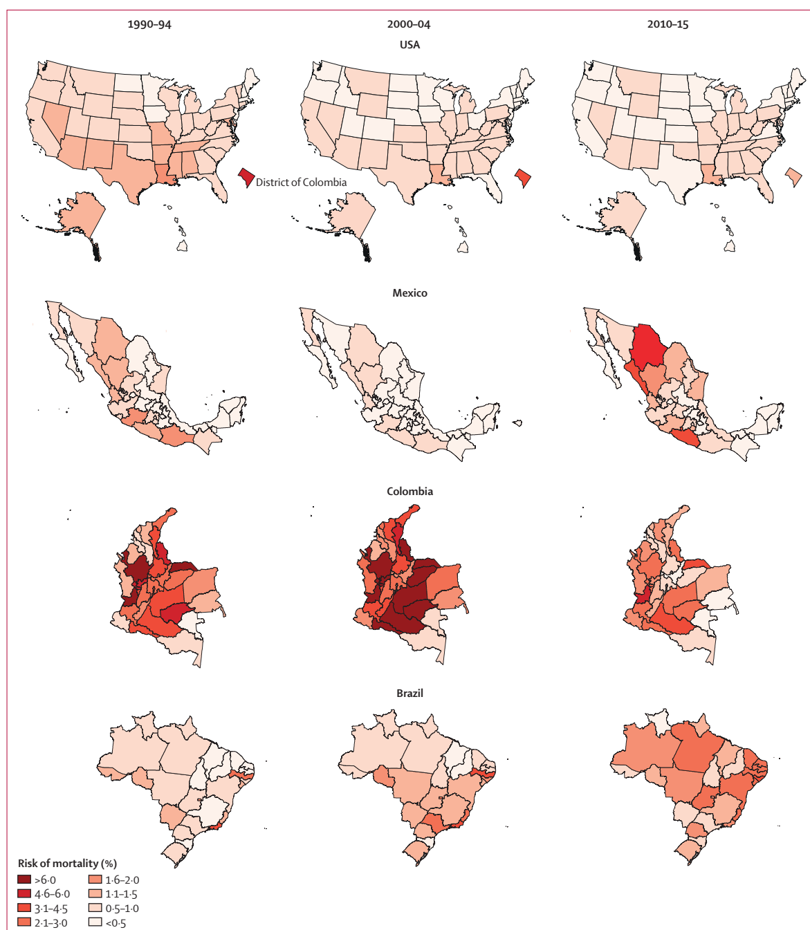
Figure 1: Subnational geographic variation in the risk of mortality from firearms in the USA, Mexico, Brazil, and Colombia among men aged 15–34 years, 1990–2015
