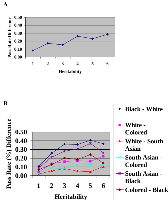
Fig. (3). Relation of heritability to mean group differences in pass rate for 6 parcels of items. (A) Canadian twins and Serbian Roma on Colored Progressive Matrices; (B) White, Asian, Colored, and Black high school students in South Africa on Standard Progressive Matrices. (Based on data from Rushton et al. [63]).
