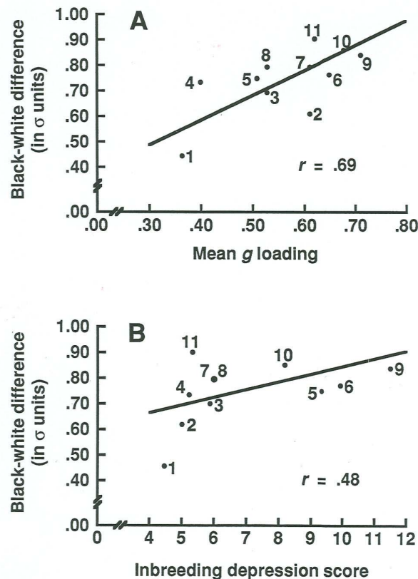
Fig. (2). Regression of Black-White differences on g loadings (Panel A) and on inbreeding depression scores (Panel B). The numbers indicate subtests from the Wechsler Intelligence Scale for Children-Revised: 1, Coding; 2, Arithmetic; 3, Picture completion; 4, Mazes; 5, Picture arrangement; 6, Similarities; 7, Comprehension; 8, Object assembly; 9, Vocabulary; 10, Information; 11, Block design. (From Rushton [23], p. 188, Figure 9.1).
